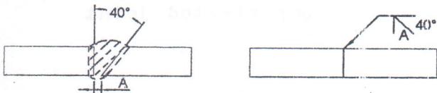
40° Single - Bevel
