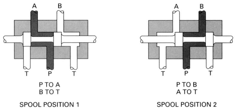
SCHEMATIC DRAWINGS
